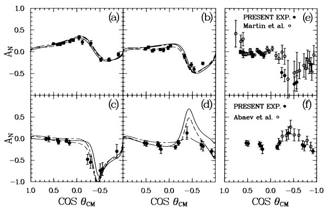
FIG. 2. (a)–(d): Analyzing power, A_N , measured in \pi^+p elastic scattering with use of transversely polarized target. The incident pion momenta are 471, 547, 625, and 687 MeV/ c , respectively. The curves are the results of the three partial-wave analyses of Ref. 10 (solid curve), Ref. 11 (dot-dashed curve), and Ref. 12 (dashed curve). (e) Results of the present experiment at 625 MeV/ c compared to the data of Martin et al. (Ref. 17) at 617 MeV/ c . (f) Results of the present experiment at 687 MeV/ c compared to the data of Abaev et al. (Ref. 18) at 685.5 MeV/ c .
