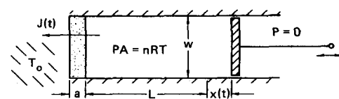
Fig. 1. Schematic diagram of the two-dimensional piston and cylinder.
