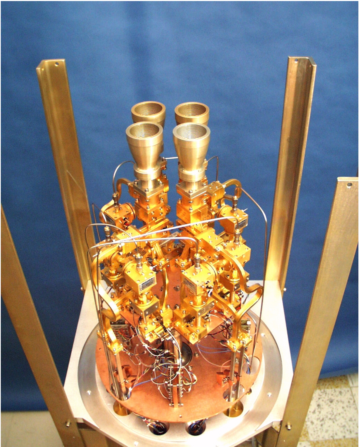
The GBT Q-band ( \nu_{\text{RF}} from 40 to 52 GHz) receiver showing the 20 K cryogenic stage with four feed horns, noise calibration sources, RF
